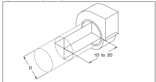
Figure 13. Straightening Vanes
