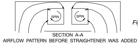
Figure 18. Duct System
